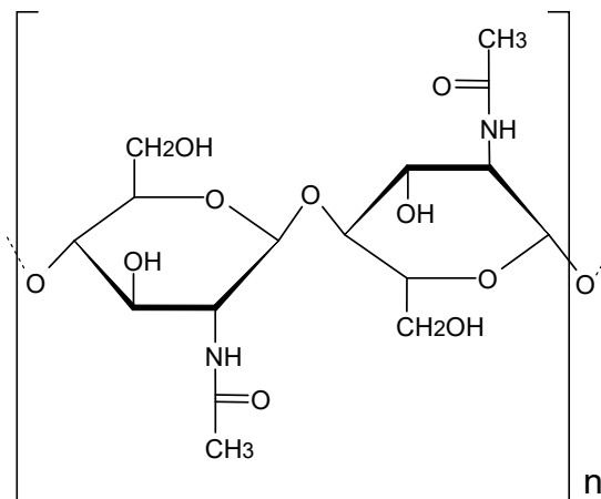
Chitine
